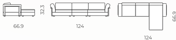
R section: 2seat+chaise(3PL)
