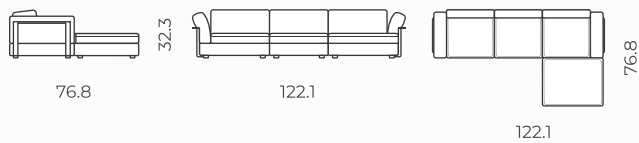
R section: 2seat+corn+seat(4PL)
